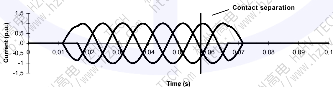
Figure 29 – Graphical representation of the three valid symmetrical breaking operations for three-phase tests in a non-solidly earthed neutral system (first-pole-to-clear factor 1,5)
