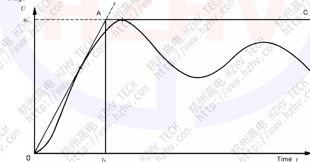
Figure E.4 – Representation by two parameters of a prospective transient recovery voltage of a circuit – Case E.2. c) 3) ii)
